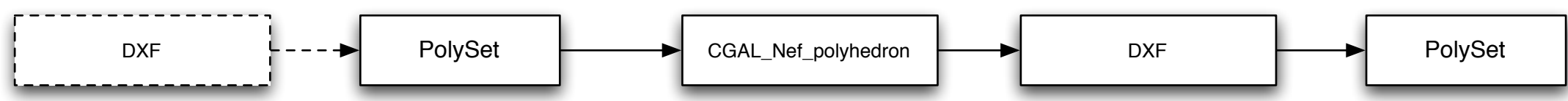
dxflinextrude.cc/dxfrotextrude.cc
