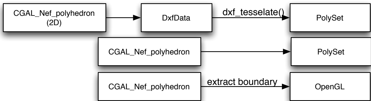
transform.cc
